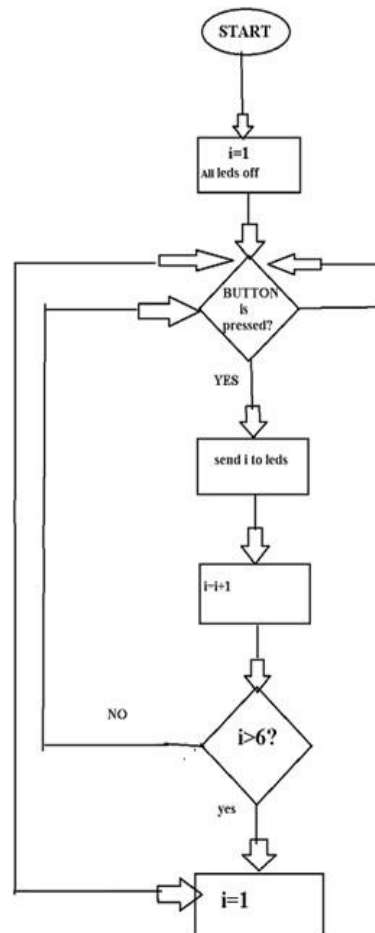
Fig.7 flow chart
