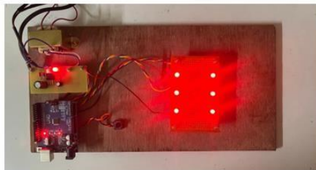
Figure 11: For the number 6 of the dice: lights up the groups 1, 2, 3, 5, 6, 7
