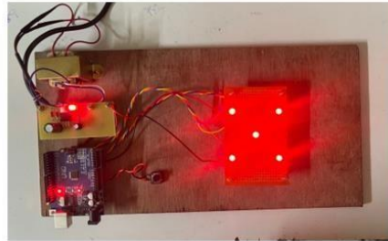
Figure 16: For the number 5 of the dice: lights up the groups 1, 2, 4, 6, 7
